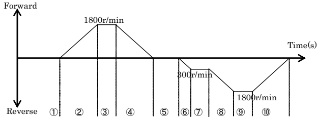
Figure 7.1 Driving Pattern
