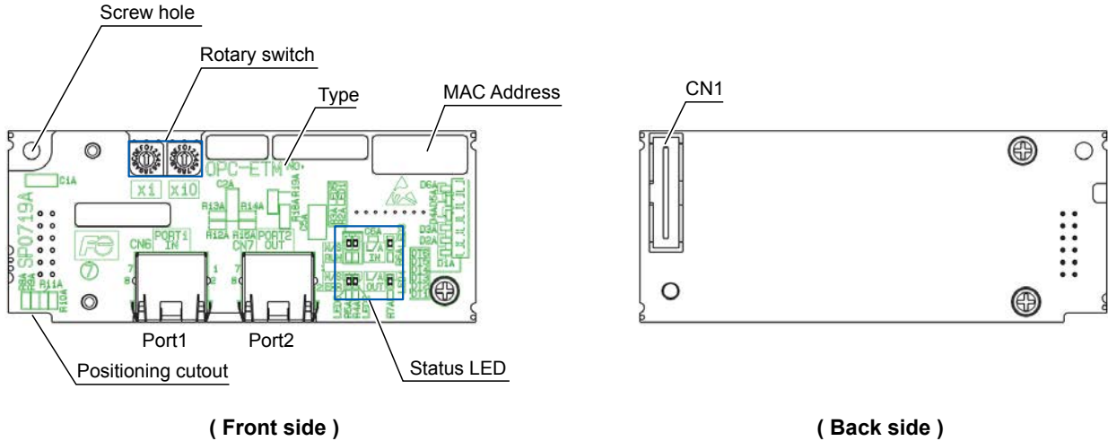
Names of Parts on Multi-protocol Ethernet Communication Card
