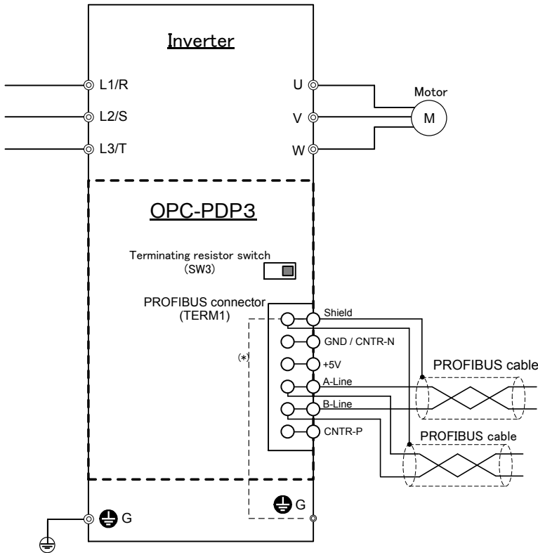
Figure 4.1 Connection Diagram
